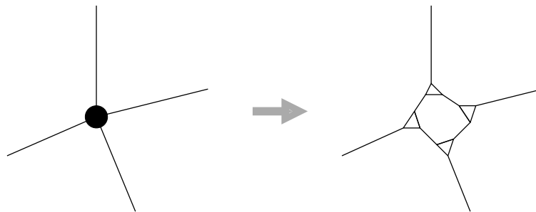
FIGURE 2. The decoration of a vertex of degree 4 in the Fisher correspondence. On the left, a vertex from the initial Ising graph. On the right, its replacement in the dimer graph.
