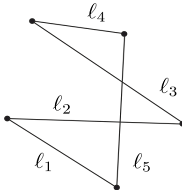
FIGURE 1. A Planar Polygon
