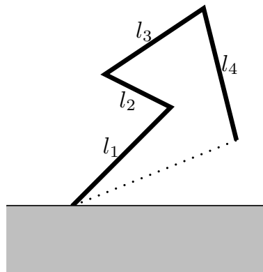
FIGURE 2. The distance map f_l is determined by the length of the dotted line.
