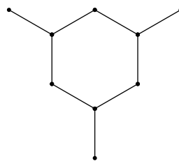
FIGURE 2. The cube complex K_2Q .
