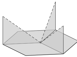
FIGURE 1. A realization of F_2Q .
