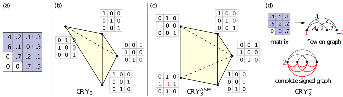
FIGURE 1. (a) A doubly-stochastic matrix in \mathcal{CRV}_4 , (b) the polytope \mathcal{CRV}_3 , (c) the polytope \mathcal{CRV}_3^{ASM} , (d) map from a matrix in \mathcal{CRV}_3 to a flow on K_4 ; graph K_4^\pm associated to \mathcal{CRV}_3^\pm .
