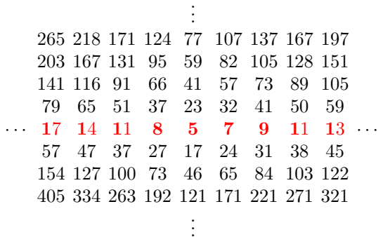
Figure 6: A more complicated tiling.
