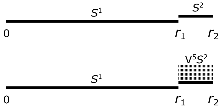
FIGURE 1. The persistent homology of \mathbf{VR}_{<}(Y; r) (top) and \mathbf{VR}_{\leq}(Y; r) (bottom) in homological dimensions 1 and 2. See Theorem 7.4 and Corollary 7.5.
