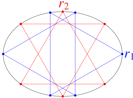
FIGURE 4. The inscribed equilateral triangles \Delta_{(\pm a, 0)} in blue have radius r_1 , and the inscribed equilateral triangles \Delta_{(0, \pm 1)} in red have radius r_2 .
