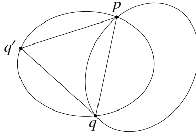
FIGURE 3. Figure for proof of Lemma 6.8
