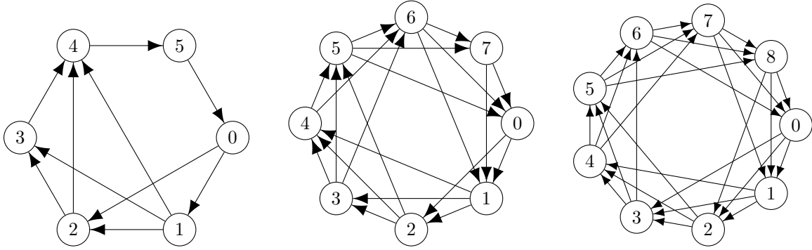
FIGURE 2. (Left) A cyclic graph of winding fraction \frac{1}{4} ; dominated vertex 1 is fast (Definition 5.8) and 3 is slow. (Middle) A cyclic graph of winding fraction \frac{1}{3} ; dominated vertex 3 is fast and 7 is slow. (Right) The cyclic graph C_9^3 .
