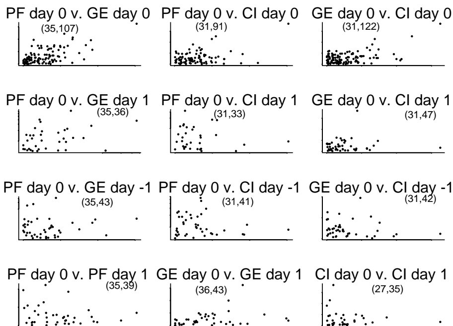
FIGURE 1. Scatterplots of standardized exceedances on unit Fréchet scale. The three stocks are Pfizer (PF), General Electric (GE) and Citibank (CI); plotted are the values on the current day (day 0) versus current day, following day (day 1) and previous day (day -1). The two numbers displayed on each plot are the actual number of joint exceedances (second number), and the expected value of the number of joint exceedances if the two variables were independent (first number). It can be seen that for all three “day 0 v. day 0” plots, there is substantial dependence between the extremes of the two series. For plots of day 0 against day 1 or day -1, however, the evidence for dependence is much less clear-cut.
