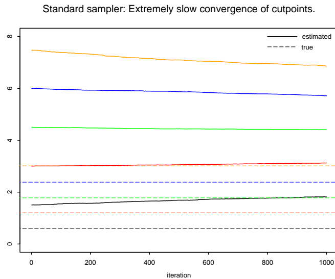
FIGURE 1. First 1000 MCMC iterations for cutpoints produced by standard Gibbs sampler. The dotted lines indicate the true values.
